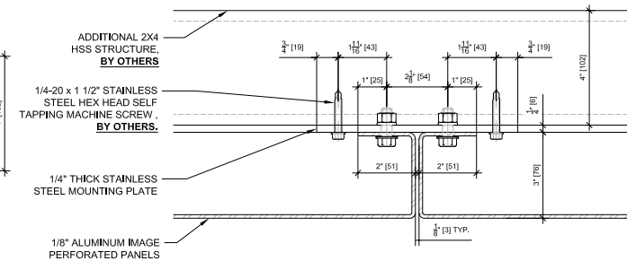
4 HORIZONTAL SECTION DETAIL AT OMEGA CHANNEL 001 SCALE: 1/2" = 1'-0"
