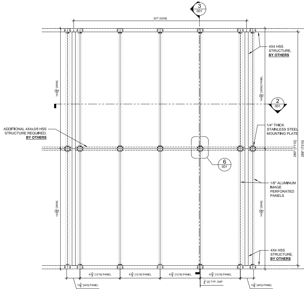
1 ELEVATION OF TYPICAL BAY 001 SCALE: 1/2" = 1'-0"
