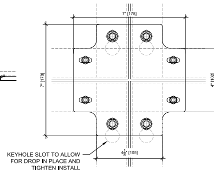
3 FRONT DETAIL OF MOUNTING PLATE 001 SCALE: 6" = 1'-0"
