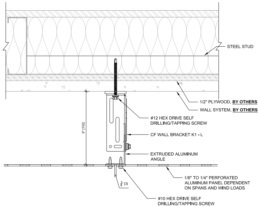
1 PLAN SECTION DETAIL 01 SCALE: 6" = 1'-0"
